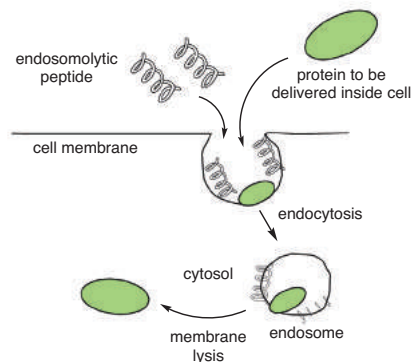
Figure 1. Two Representative Approaches of Cytosolic Protein Delivery. (a) By Conjugation with a Cell-Penetrating Peptide (CPP): (i) Protein May Permeate through the Cell Membrane, or (ii) Is Taken Up by the Cell via Endocytosis, Followed by Endosomal Escape to Reach the Cytosol. (b) Cytosolic Protein Delivery Is Also Possible by Incubating the Protein with Endosomolytic Peptides. (Ref. 9,10)
